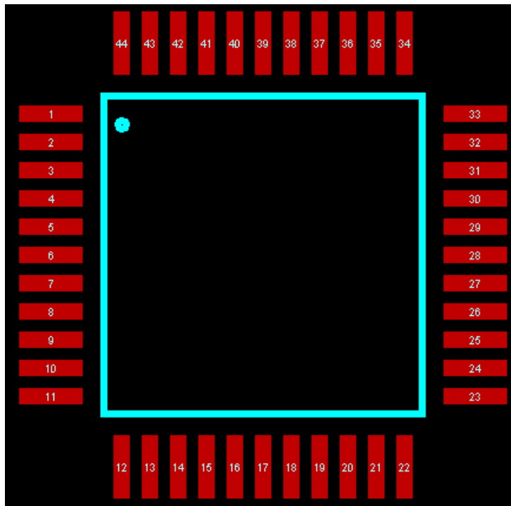
Finished SQFP44
