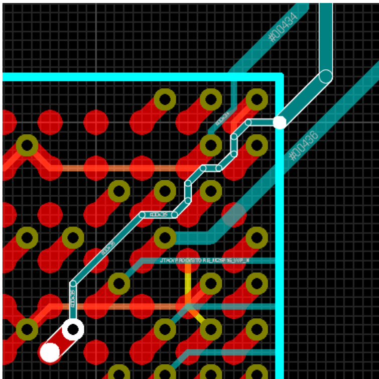
Advanced necking: The SHIFT key is held down while routing the escape from the BGA and then released to resume routing at normal track width.
