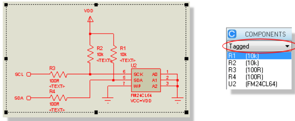
Components selected in Proteus and shown in the Layout - Component 'tagged' mode
