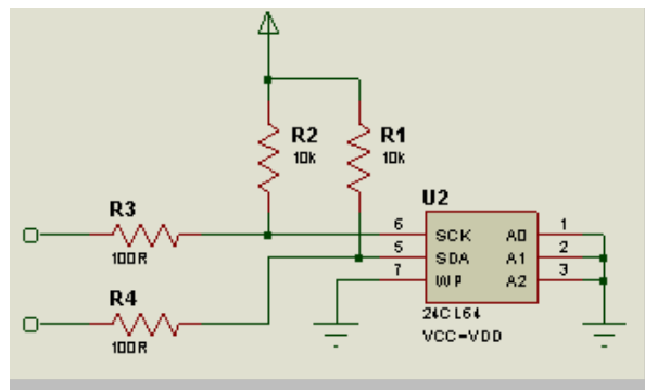
Schematic section with all parts / terminals placed
