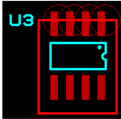
U3 with a Keepout
