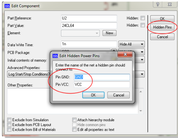
Hidden Power pins in schematic components.
