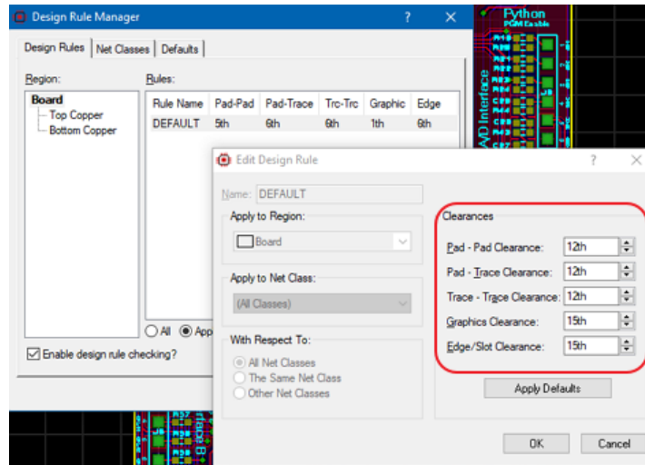
Default clearance settings in the DRC manager
