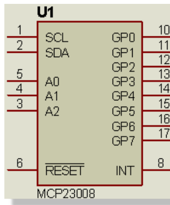
The MCP23008 Completed
