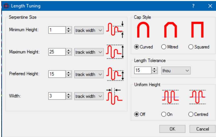
Configuring Length Matching Options.
