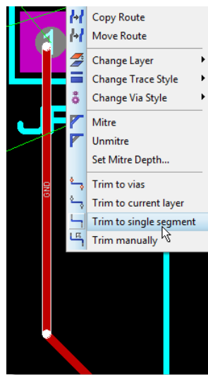
Trimming a trace to a single segment
