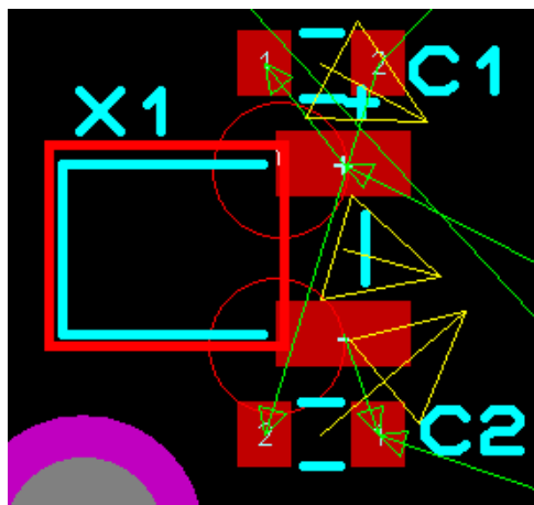
Keepout placed produces 2 DRC errors
